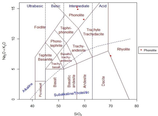
Figure 6: TAS diagram for Yelwa phonolites (After Le Bas et al. , 1986)
