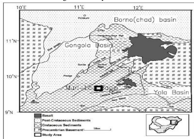
Figure 1: Geological map of the Northern Benue Trough showing the study area (Modified from Zaborski et al. , 1997)
