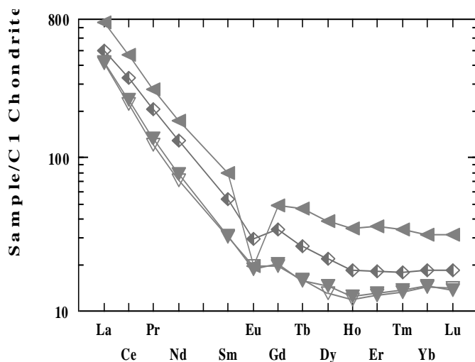
Figure 14: Chondrite-normalized REE pattern of Yelwa Phonolites. [Normalizing values were those of Taylor and McLennan, (1985)].
