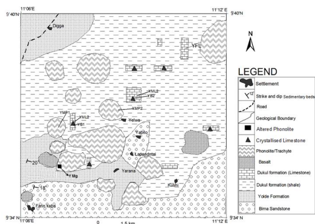
Figure 2: Geological map of Yelwa area
