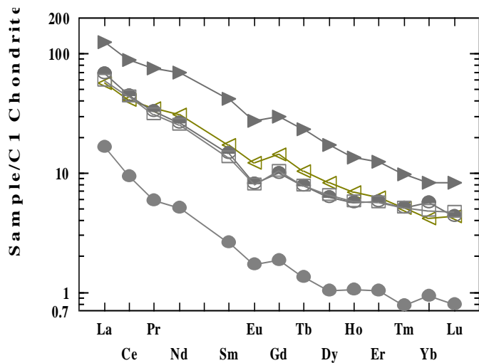
Figure 3: Chondrite-normalized REE pattern of limestone of Yelwa study area. [Normalizing values were those of Taylor and McLennan, (1985)].
