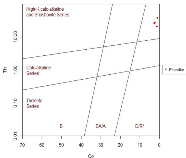
Figure 12: Co vs Th bivariate diagram for Yelwa phonolites (After Hastie et al., 2007).
