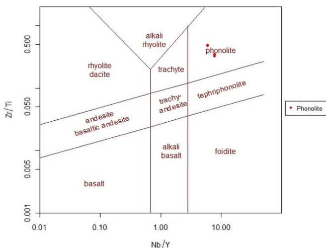
Figure 11: Nb/Y vs Zr/Ti bivariate diagram for Yelwa phonolites (After Pearce, 1996).
