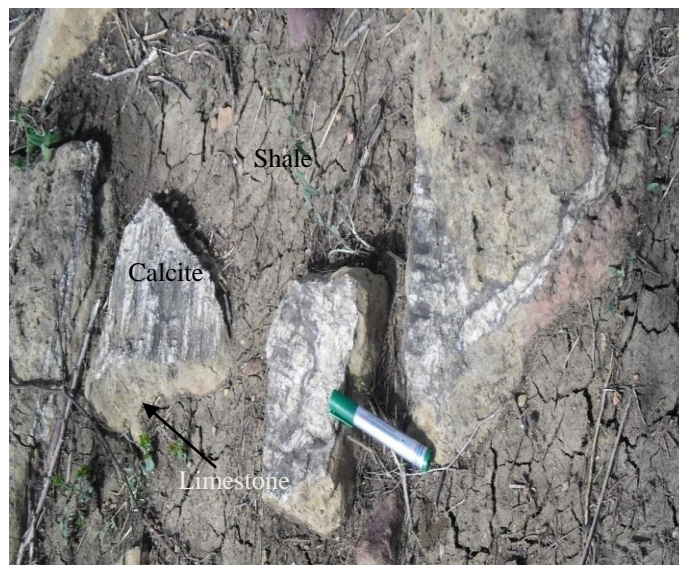
Plate 1: Recrystallized Calcite, Limestone and Shale of Dukul Formation (N9°36.694' and 11°07.859')
