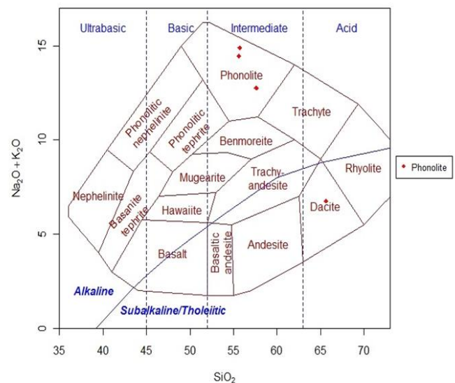
Figure 5: TAS diagram for Yelwa phonolites (After Cox et al. , 1979)
