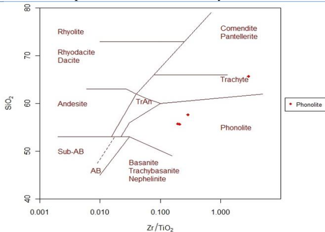
Figure 7: Zr/TiO 2 – SiO 2 diagram for Yelwa phonolites (After Winchester and Floyd, 1977).
