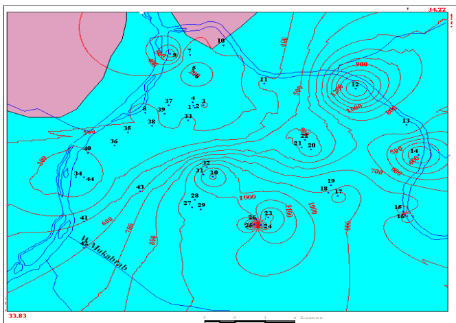
Figure (3) spatial distribution of TDS in the study area
