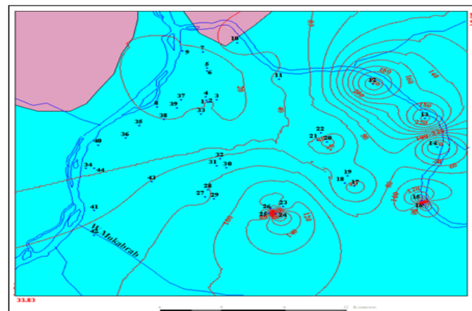
Figure (6) spatial distribution of Sulphate in the study area
