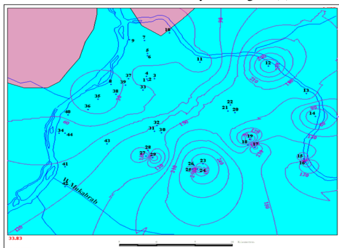
Figure (4) spatial distribution of sodium in the study area
