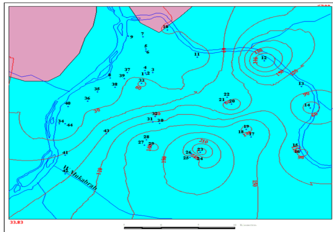
Figure (7) spatial distribution of chloride in the study area
