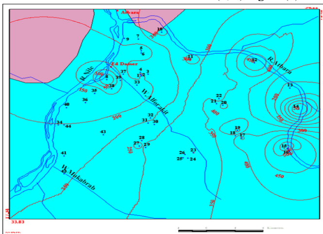
Figure (5) spatial distribution of bicarbonate in the study area
