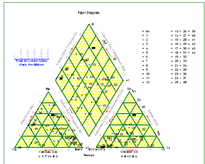
Figure (8) piper diagram me in study area
